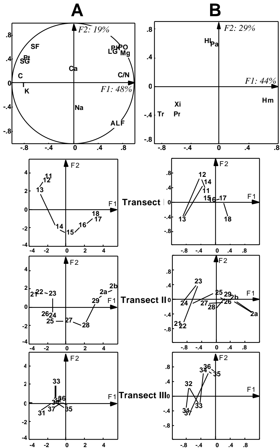
Figure 4 : Results of the soil data PCA (1A) and of the nematological data CA (1B). Top: F1 X F2 factor planes of the columns (PCA correlation circle of the soil variables and CA factor plane of the six nematode species). Bottom : F1 X F2 factor planes of the rows (left = PCA, right = CA); the three transects have been represented separately and sampling points are numbered 11 to 18, 21 to 2b and 31 to 37; cf. table legends.
