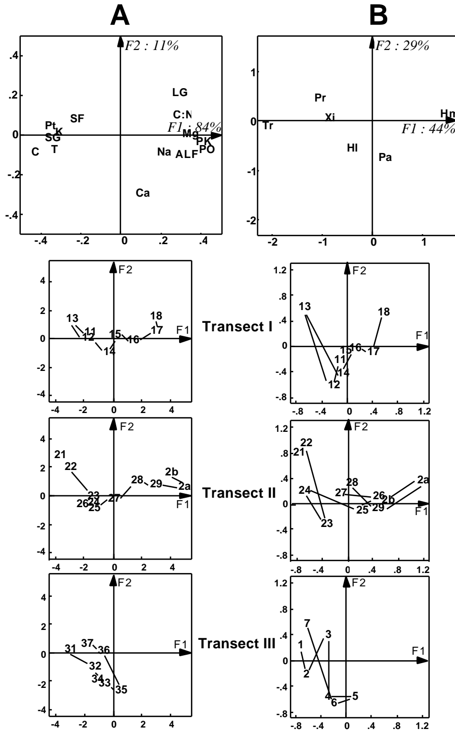
Figure 5 : Co-structure analysis. Top : F1 X F2 factor planes of the columns (A : soil variables; B : nematode species). Bottom : F1 X F2 factor planes of the rows (cf. figure 2 and tables legends).
