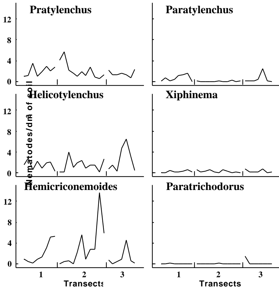
Figure 3 : Representation of the six nematode species abundance ( \times 10^{-3} ) along the three transects.
