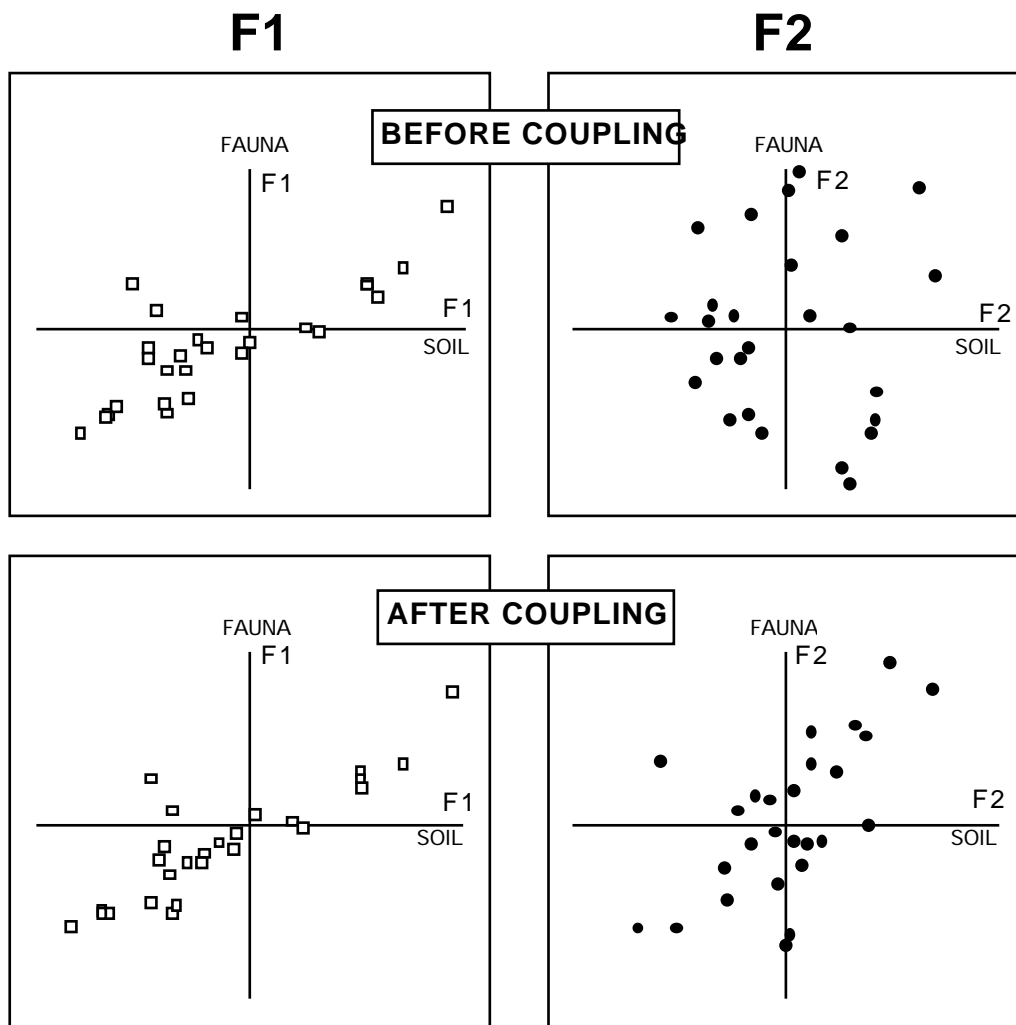
Figure 6 : For each sampling point, projection, before and after coupling, of the first (□) and second (●) factor scores of the analyses of soil and nematological data. Before coupling: the first factor of CA has been plotted against the first factor of PCA (left); the second factor of CA has been plotted against the second factor of PCA (right). After coupling: the first factor of the co-inertia analysis of nematological data has been plotted against the first factor of the co-inertia analysis of soil data (left); the second factor of the co-inertia analysis of nematological data has been plotted against the second factor of the co-inertia analysis of soil data (right).
