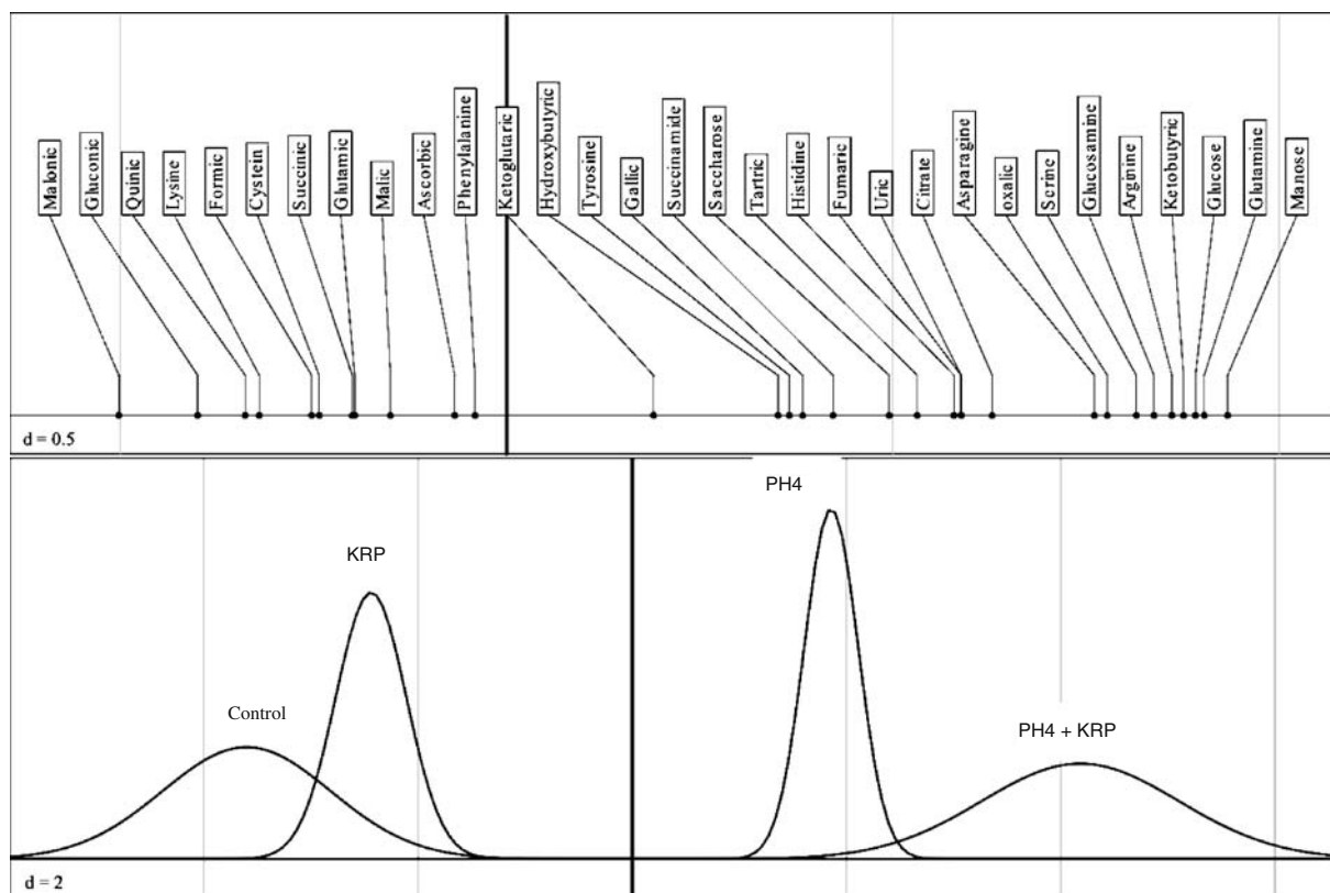
Fig. 2 Graphical display (biplot) of BGA axes showing the Substrate Induced Respirations with respect to the soil treatments. The upper and medium parts of the figure show the scores of the 31 substrates on the first and second BGA axes, respectively. The four Gauss curves in the medium and lower parts of the figure represent the mean and the variance of the scores of the soil samples on the first and second BGA axes.
