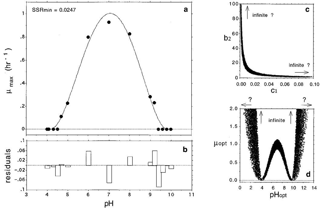
FIG. 4. (a) Fit of equations 1' and 2' with the data set of Petran and Zottola (the two models gave the same fit). (b) Plot of the residuals (observed-calculated). (c and d) Two examples of the high correlations observed with the models between two of the parameters. (c) Correlation between b_2 and c_1 for equation 1' (10,000 points were computed). (d) Correlation between pH_{opt} and \mu_{opt} for equation 2' (20,000 points were computed). The extents of the correlations seem to be infinite.
