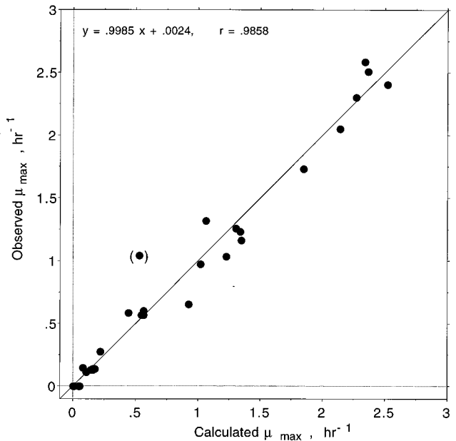
FIG. 5. \mu_{max} values calculated with the CTPM versus observed \mu_{max} values for E. coli O157:H7. The equation and the line were obtained by linear regression ( r is the correlation coefficient). The experimental value in parentheses observed at 28°C and pH 4.5 seems to be an outlier.
