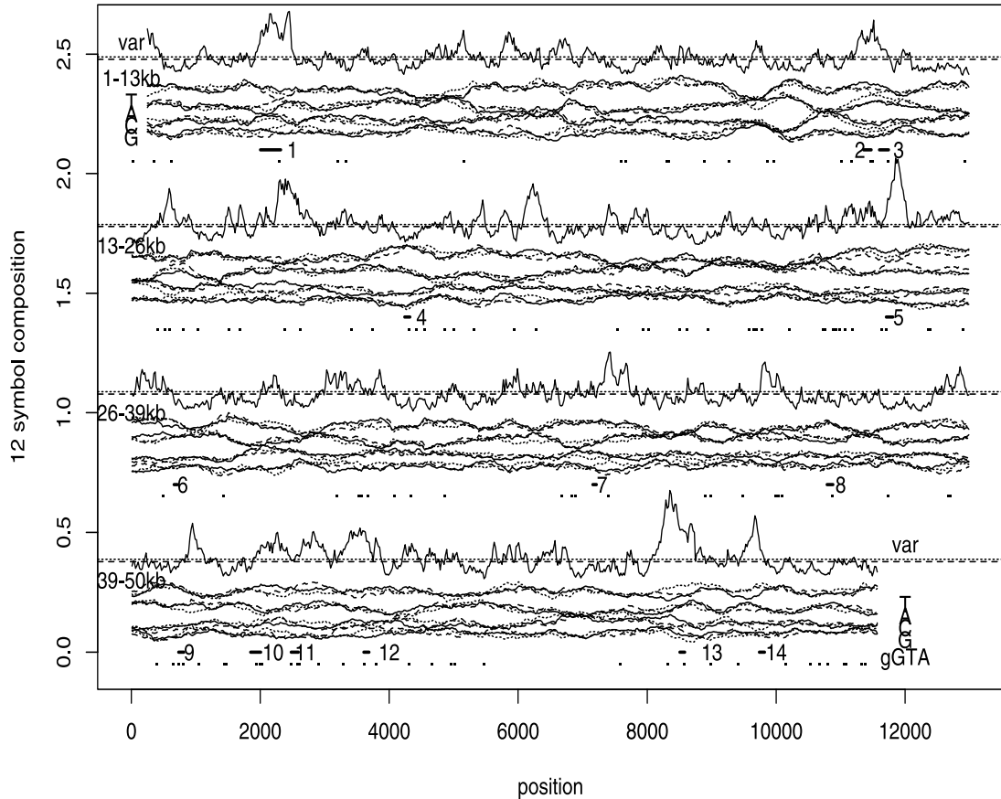
Fig. 9. The human protein kinase chk2 gene (on chromosome 22, 14 exons, sequence length N = 50,824 bases). The following information is shown: base compositions in three separate phases in a moving-window (window length = 500 bp, moving distance = 20 bp) G1%, G2%, G3%, etc.; variance by Eq. (6); location of 14 exons, matches with the pattern GGTA. Exon regions tend to have larger variances.
