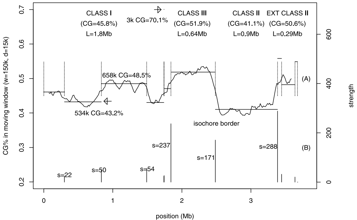
Fig. 1. Eleven domains segmented at s_0 = 20 for MHC sequence. Sequence length is N = 3,673,778 bases. (A) G + C% in a moving window (window size is 150 kb, and moving distance 15 kb); domain borders (vertical dashed lines); and G + C% in segmented domains (horizontal solid lines). (B) Segmentation strength s (vertical bars). The four known isochores (telomere is on the left side and centromere on the right side) class-I, -III, -II, and extended class-II, and the isochore border between class-III and -II are marked in the plot.
