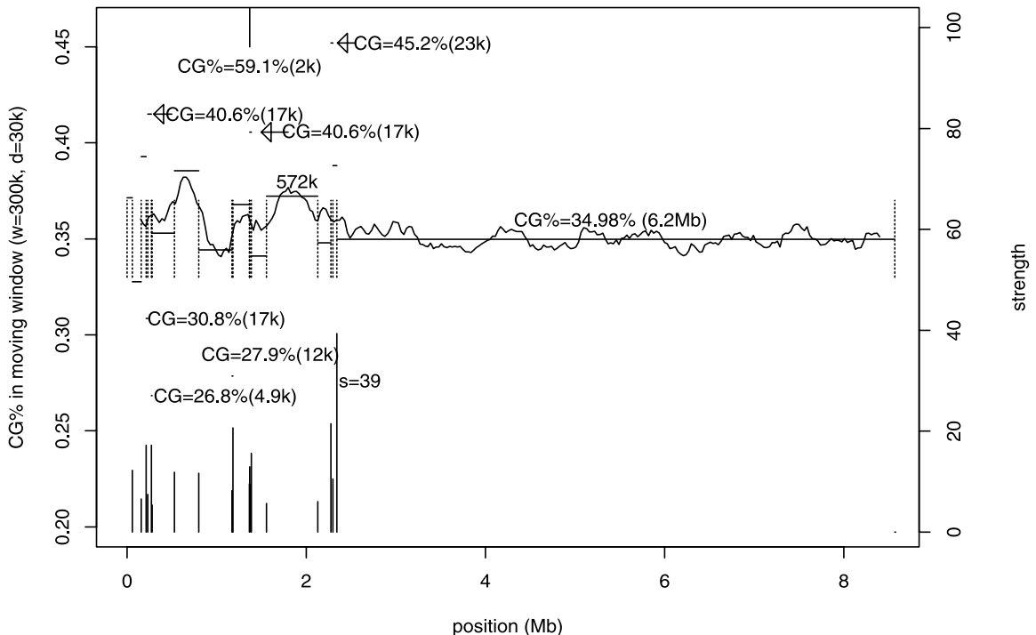
Fig. 3. Nineteen domains segmented at s_0 = 5 for the longest contig of chromosome 1 of C. elegans (see the caption of Fig. 1 for an explanation of the plot).
